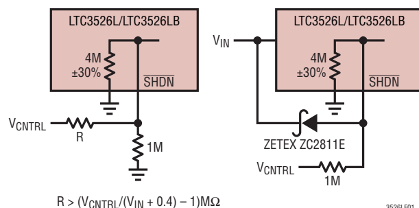
Figure 1. Recommended Shutdown Circuits when Driving \text{SHDN} above V_{IN}
