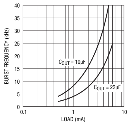
Light Load Burst Frequency vs Load
