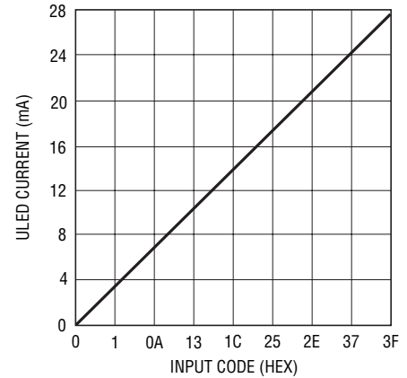
ULED Current vs Input Code
