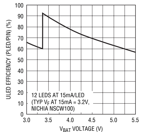
12-LED ULED Display Efficiency vs V_{BAT} Voltage
