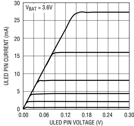
ULED Pin Current vs ULED Pin Voltage
