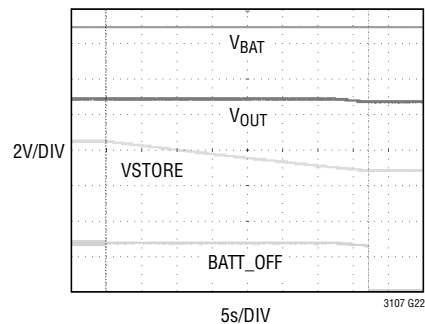
V_{STORE} Holding-Up V_{OUT} ( V_{BAT} = 3\text{V} , C_{STORE} = 1300\mu\text{F} , I_{OUT} = 50\mu\text{A} , Holdup = 37 SEC)
