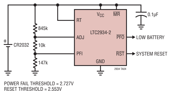
Coin Cell Voltage Monitor
