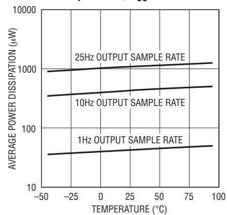
Average Power Dissipation vs Temperature, VCC = 3V
