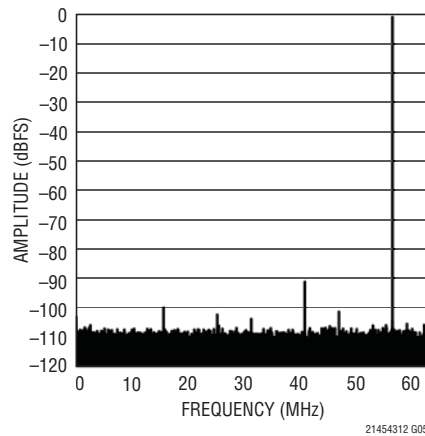
LTC2145-12: 64k Point FFT, f_{IN} = 70\text{MHz} , -1\text{dBFS} , 125Msps
