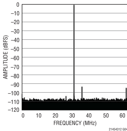
LTC2145-12: 64k Point FFT, f_{IN} = 30\text{MHz} , -1\text{dBFS} , 125Msps
