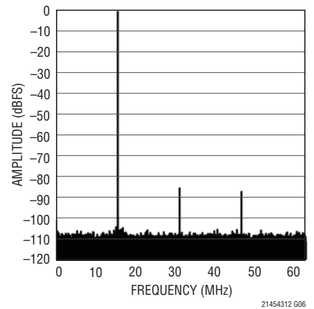
LTC2145-12: 64k Point FFT, f_{IN} = 140\text{MHz} , -1\text{dBFS} , 125Msps
