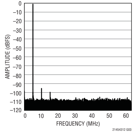
LTC2145-12: 64k Point FFT, f_{IN} = 5\text{MHz} , -1\text{dBFS} , 125Msps
