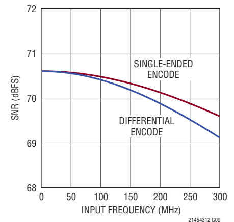
LTC2145-12: SNR vs Input Frequency, -1\text{dBFS} , 125Msps, 2V Range
