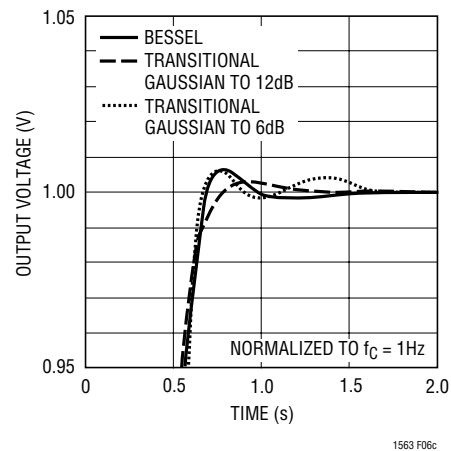
Figure 6c. Step Response—Settling
