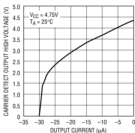
Carrier Detect Output High Voltage vs Output Current
