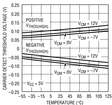
Carrier Detect Threshold Voltage (Output High) vs Temperature
