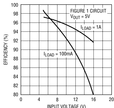
5V Efficiency vs Input Voltage
