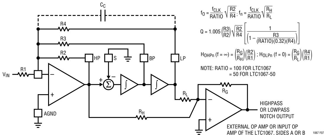
Figure 7. Mode 3a, 2nd Order Filter Providing a Highpass Notch or Lowpass Notch Output
