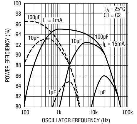
Power Efficiency vs Oscillator Frequency, V^+ = 10V
