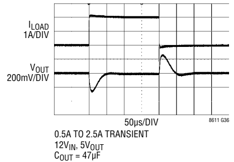
Transient Response
