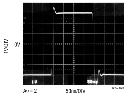
Large Signal Response, V_S = \pm 5V
