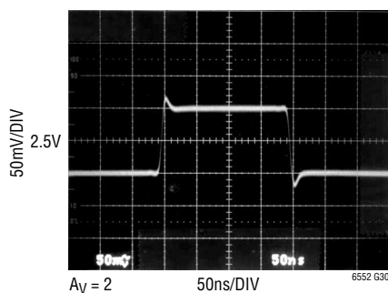
Small Signal Response, V_S = 5V, 0V
