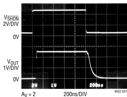
Shutdown Response
