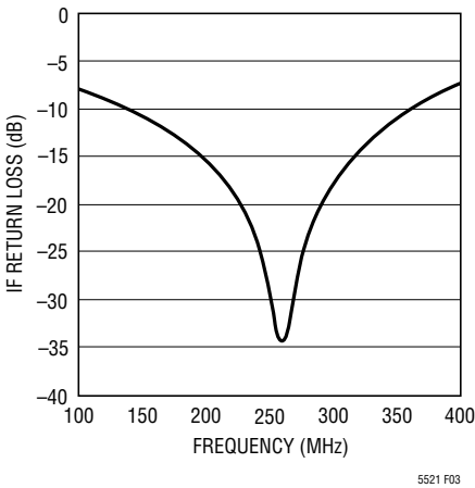
Figure 3. IF Input Return Loss
