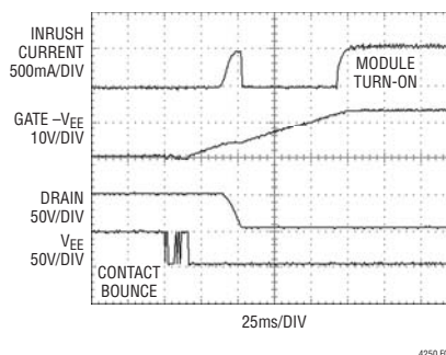
Figure 6b. Inrush Control Waveforms
