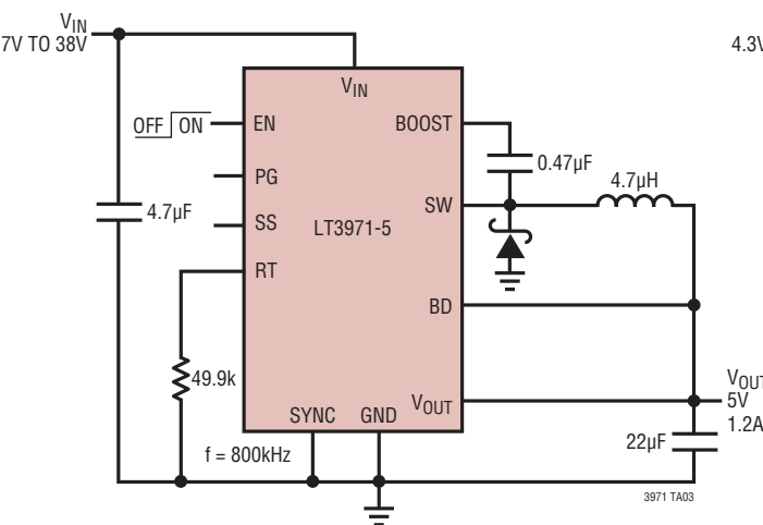
5V Step-Down Converter
