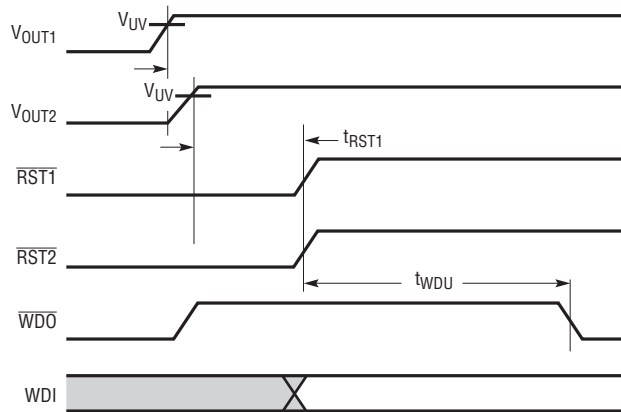
STARTUP TIMING ( V_{\text{CONFIG}} = \text{LOW} )
