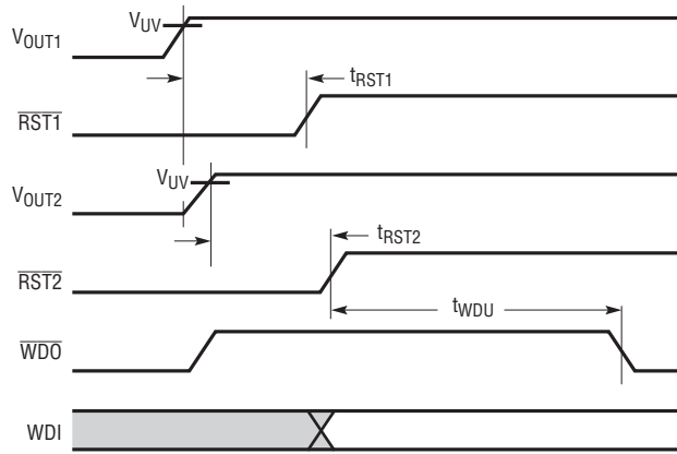
STARTUP TIMING ( V_{\text{CONFIG}} = \text{HIGH} )
