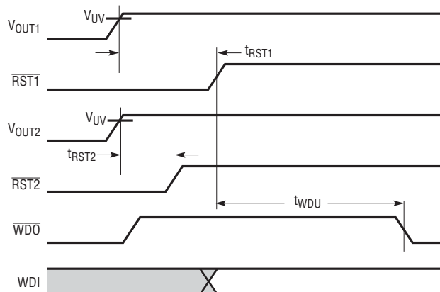
STARTUP TIMING ( V_{\text{CONFIG}} = \text{OPEN} )
