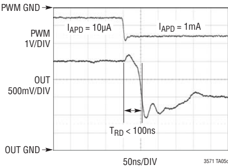
Transient Response on Input Signal Falling Edge (10µA to 1mA)
