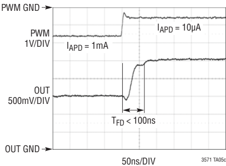
Transient Response on Input Signal Falling Edge (1mA to 10µA)
