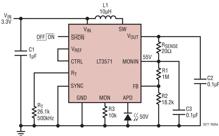
3.3V to 50V APD Bias Power Supply
