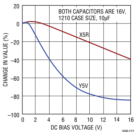
Figure 12. Ceramic Capacitor DC Bias Characteristics
