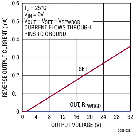
Reverse-Output Current
