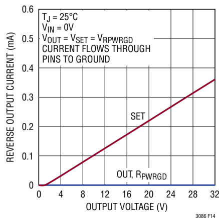
Figure 14. Reverse-Output Current
