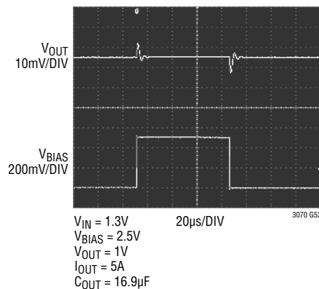
Bias Voltage Line Transient Response
