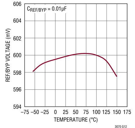
REF/BYP Pin Voltage vs Temperature
