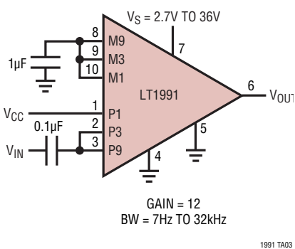
Single Supply AC Coupled Amplifier
