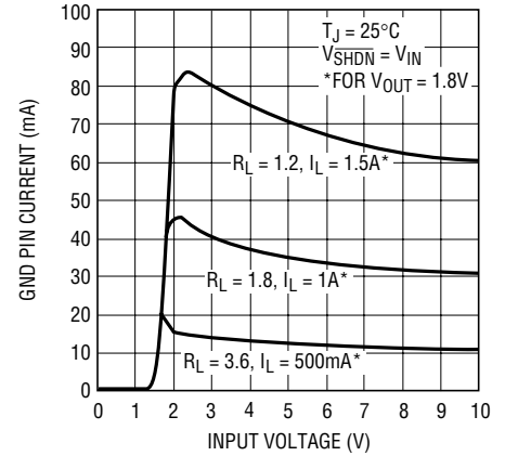
LT1963-1.8 GND Pin Current
