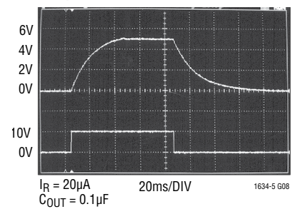
Response Time
