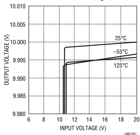
LT1460S3-10V Line Regulation
