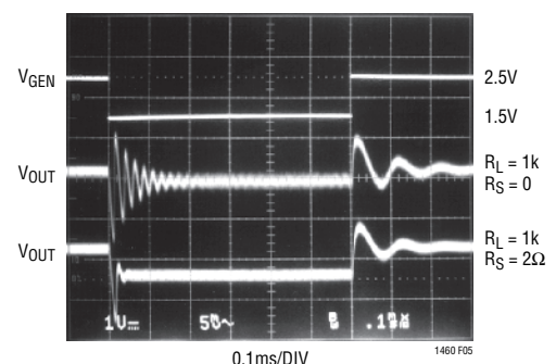
Figure 5. Effect of R_S for C_L = 1\mu F
