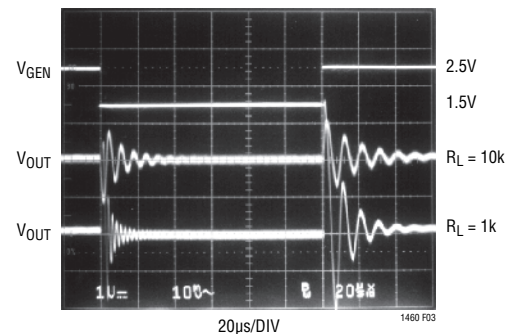
Figure 3. C_L = 0.01\mu F
