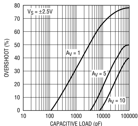
LT1218 Capacitive Load Handling
