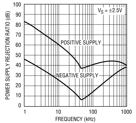
LT1219 Power Supply Rejection Ratio vs Frequency
