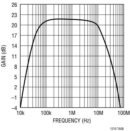
Frequency Response
