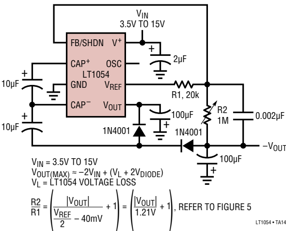
Negative Doubler with Regulator
