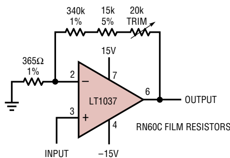
Gain 1000 Amplifier with 0.01% Accuracy, DC to 5Hz
