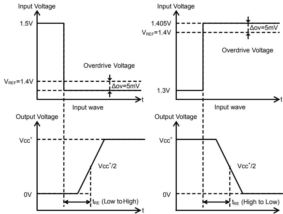
Figure 50. Response Time
