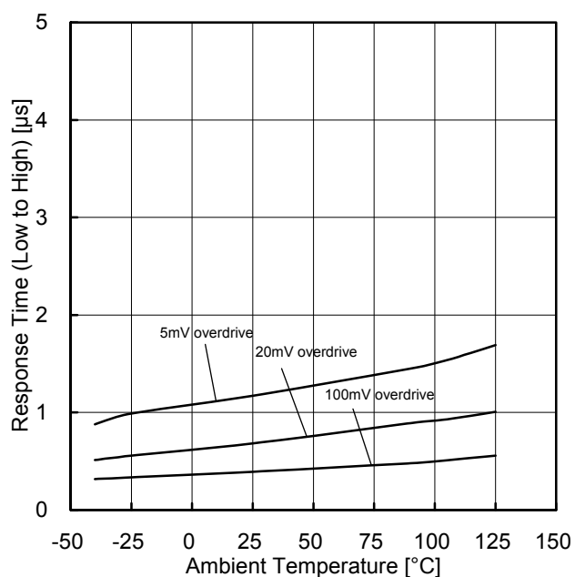
Figure 45. Response Time (Low to High) vs Ambient Temperature ( V_{CC+}=5\text{V} , V_{RL}=5\text{V} , R_L=5.1\text{k}\Omega )
