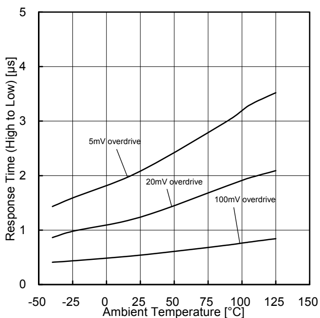
Figure 47. Response Time (High to Low) vs Ambient Temperature ( V_{CC+}=5\text{V} , V_{RL}=5\text{V} , R_L=5.1\text{k}\Omega )
