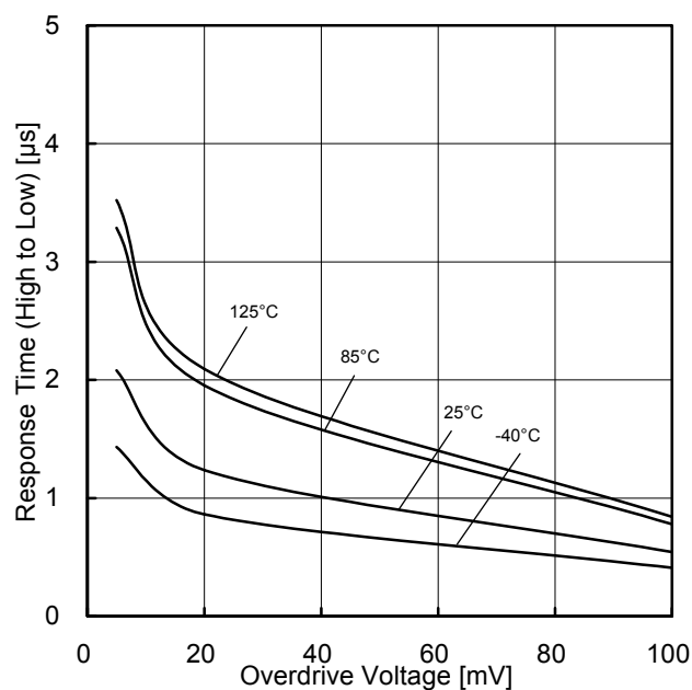
Figure 46. Response Time (High to Low) vs Overdrive Voltage ( V_{CC+}=5\text{V} , V_{RL}=5\text{V} , R_L=5.1\text{k}\Omega )
