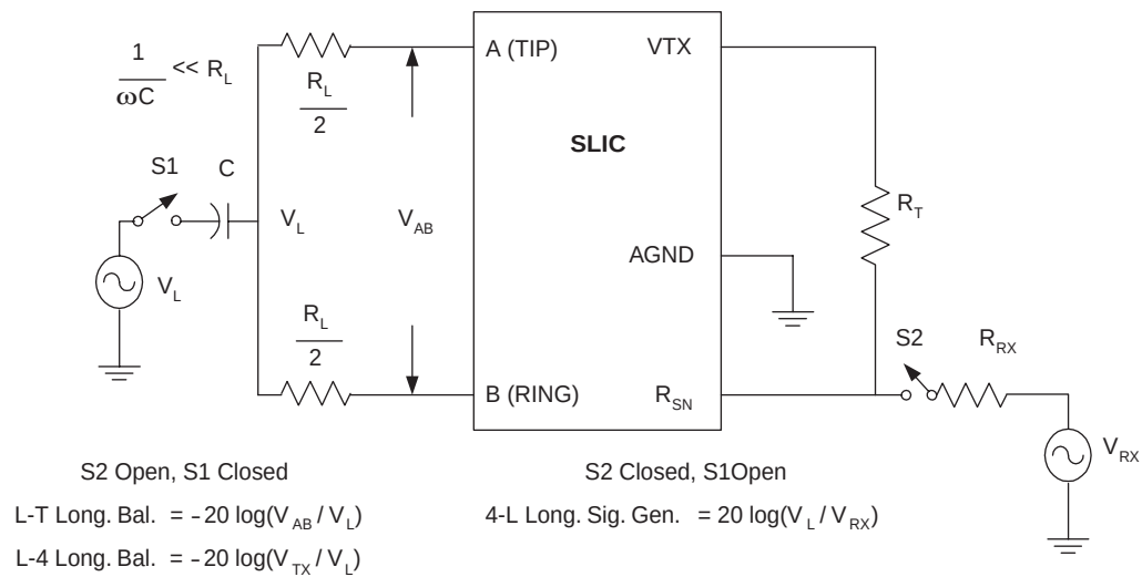
Figure 8. Longitudinal Balance
