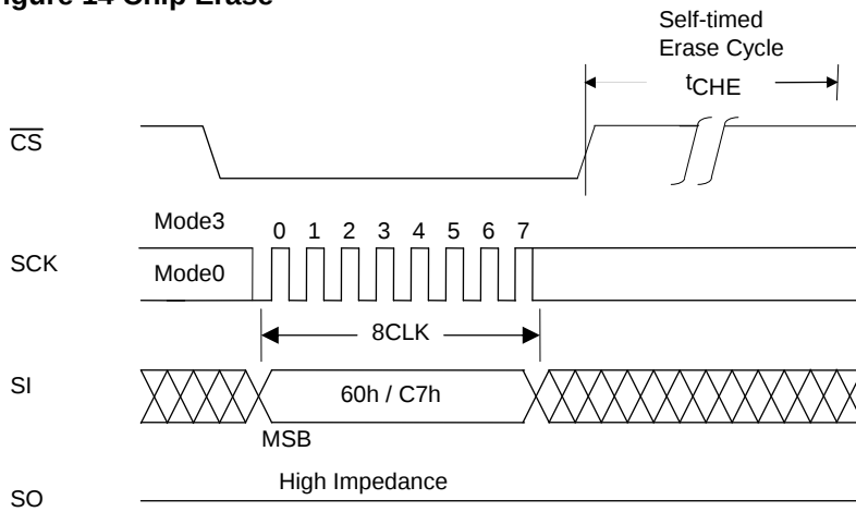
Figure 14 Chip Erase
