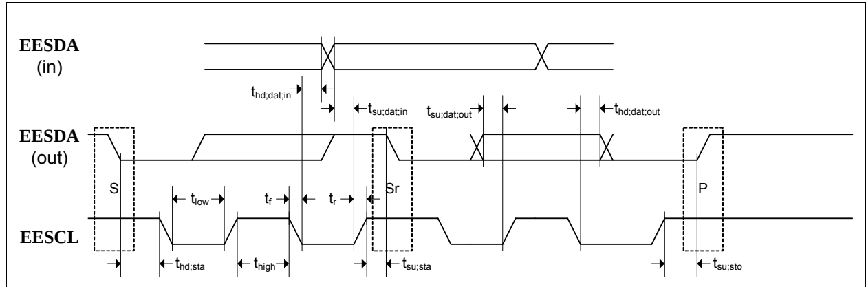
FIGURE 13-1: I 2 C MASTER TIMING DIAGRAM
