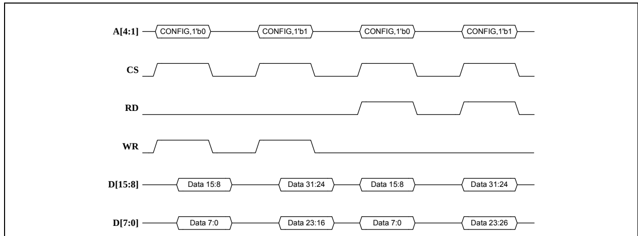
FIGURE 9-25: INDEXED ADDRESSING CONFIGURATION REGISTER ACCESS - 16-BIT WRITE/ READ
