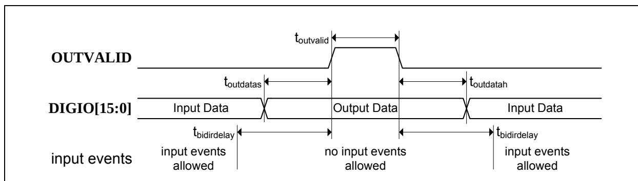
FIGURE 12-4: ETHERCAT DIGITAL I/O BI-DIRECTIONAL TIMING DIAGRAM
