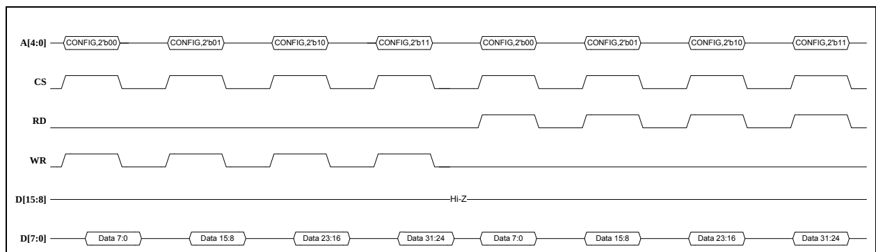
FIGURE 9-26: INDEXED ADDRESSING CONFIGURATION REGISTER ACCESS - 8-BIT WRITE/ READ
