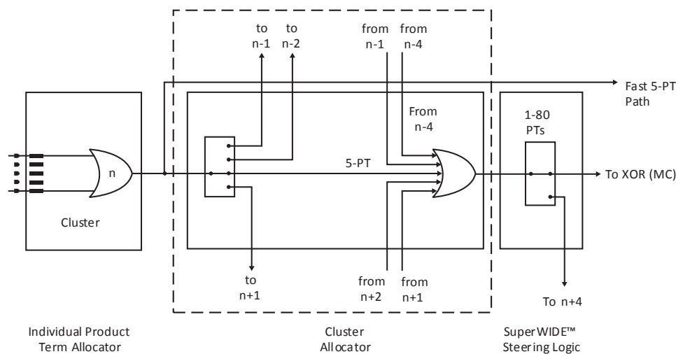
Figure 4.3. Macrocell Slice
