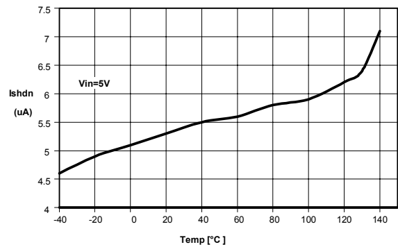
Figure 5. Shutdown Current vs. Junction TemperatureAPPLICATION INFORMATIONS
