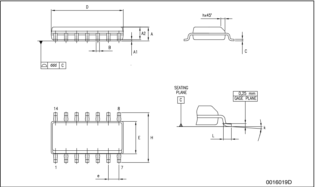
Figure 56. Package dimensions
