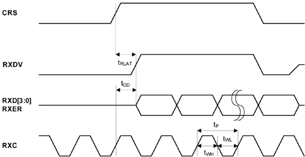
Figure 11. MII Receive Timing (10Base-T)
