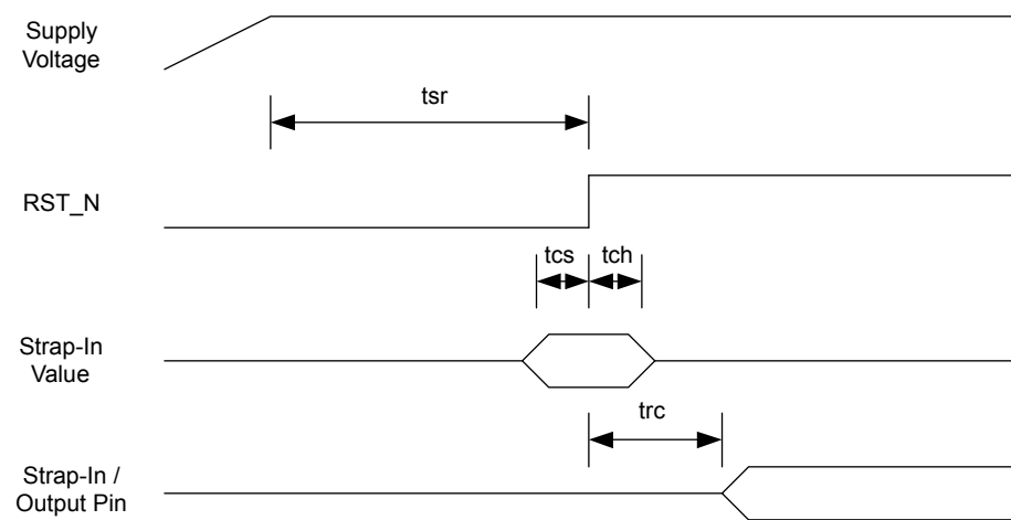
Figure 15. Reset Timing
