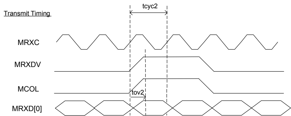
Figure 12. SNI Output Timing
