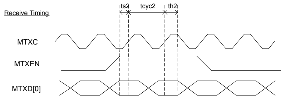
Figure 11. SNI Input Timing
