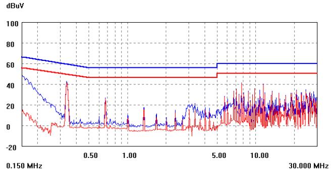
Figure 17. KHHD002A5B Vin+ Line EMC signature using above filter, Vin=48V, Blue=PK, Red=Avg.
