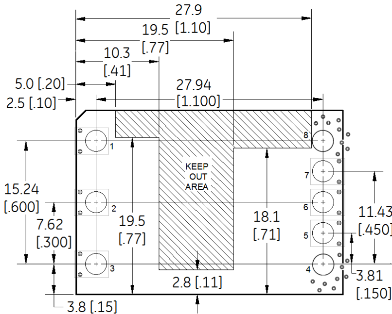
Surface Mount Pad Layout
