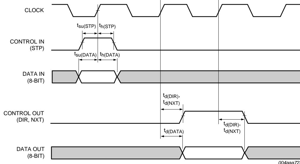
Fig 33. ULPI interface timing
