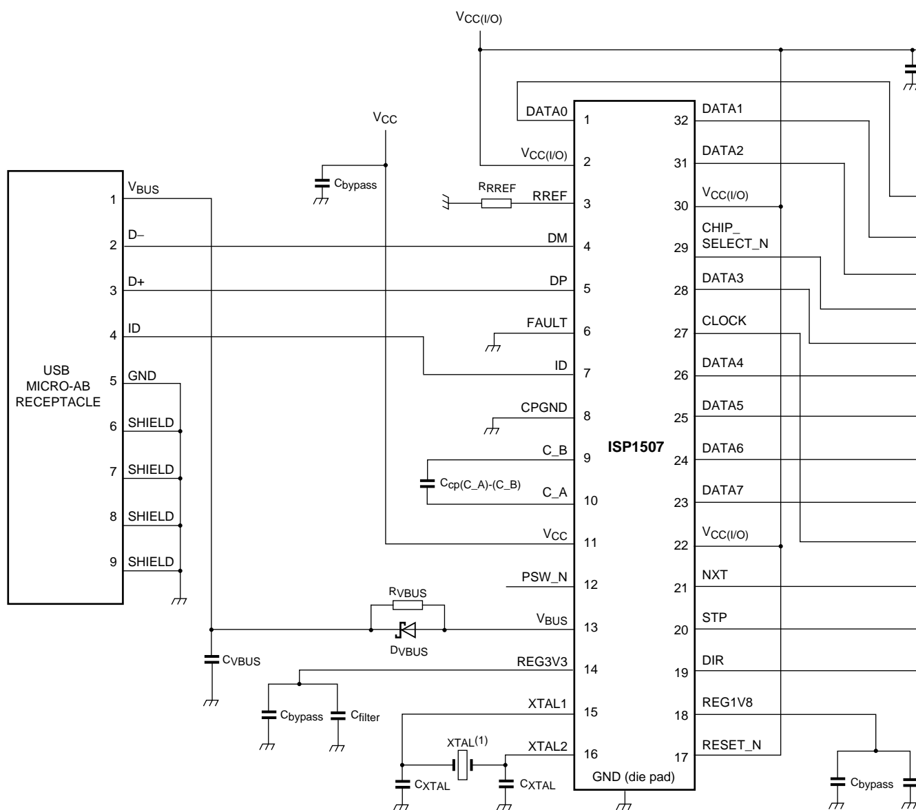
Fig 34. Using the ISP1507 with an OTG controller; internal charge pump is utilized and crystal is attached
