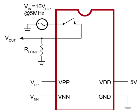
OFF Isolation
