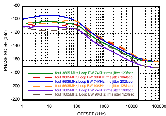
Figure 2. Typical Closed Loop Fractional Phase Noise [1] Loop Filter Configuration Table
