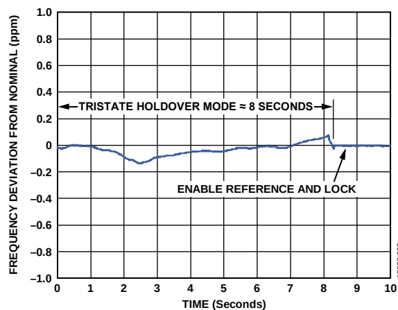
Figure 38. Frequency Deviation from Nominal vs. Time of Tristate Holdover Entry and Exit When the Phases Cross Zero
