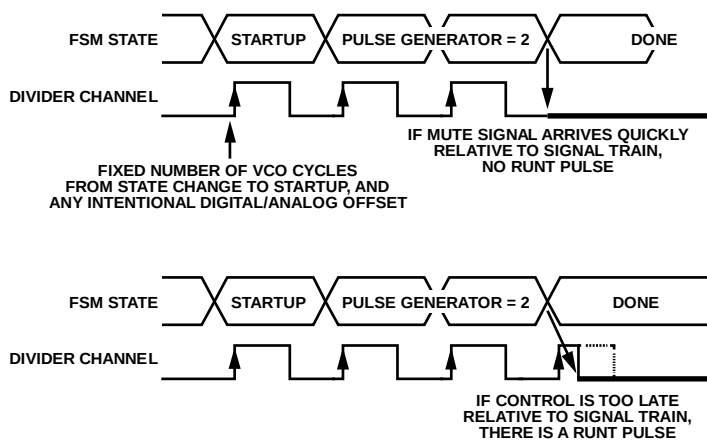
Figure 46. Start-Up Behavior of an Example Divider Configured as a Pulse Generator
