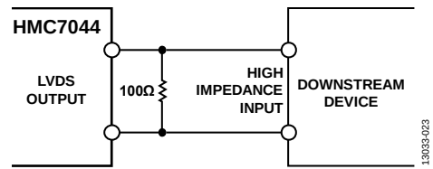
Figure 31. DC-Coupled LVDS Output Driver
