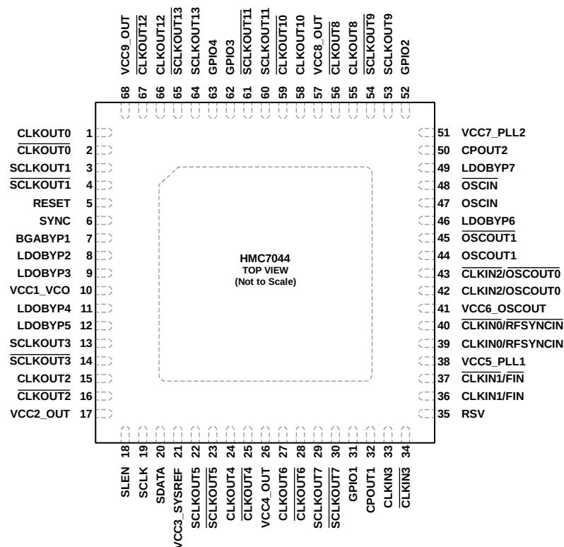
Figure 2. Pin Configuration
