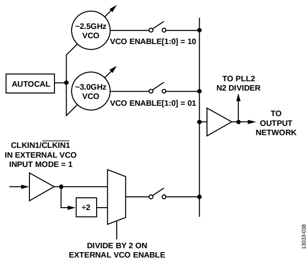
Figure 43. VCO Input Network
