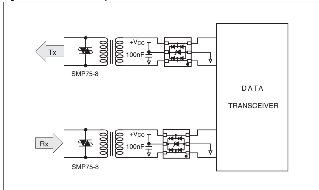
Figure 13. T1/E1/Ethernet protection
