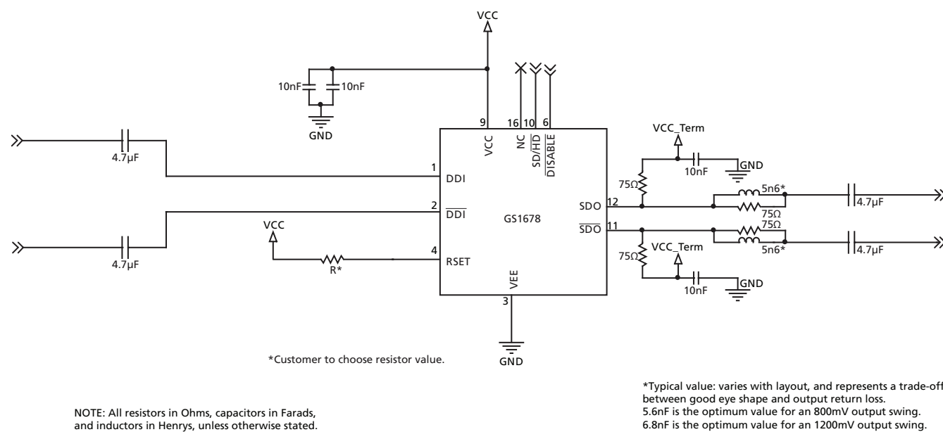
Figure 4-1: Typical Application Circuit
