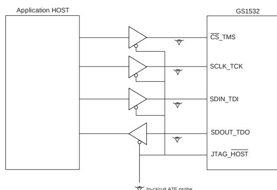
Figure 3-11: In-Circuit JTAG
