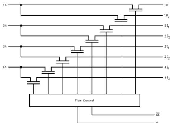
Figure 1. Logic Diagram
