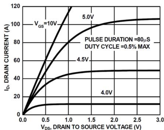
Figure 8. Saturation Characteristics
