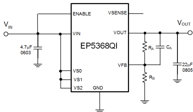
Figure 7. Applications Circuit for Operation at 700mA
